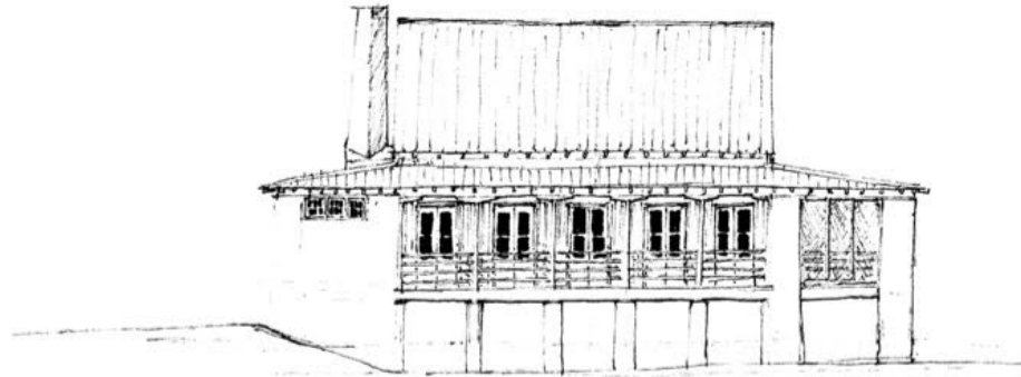
SIDE ELEVATION
